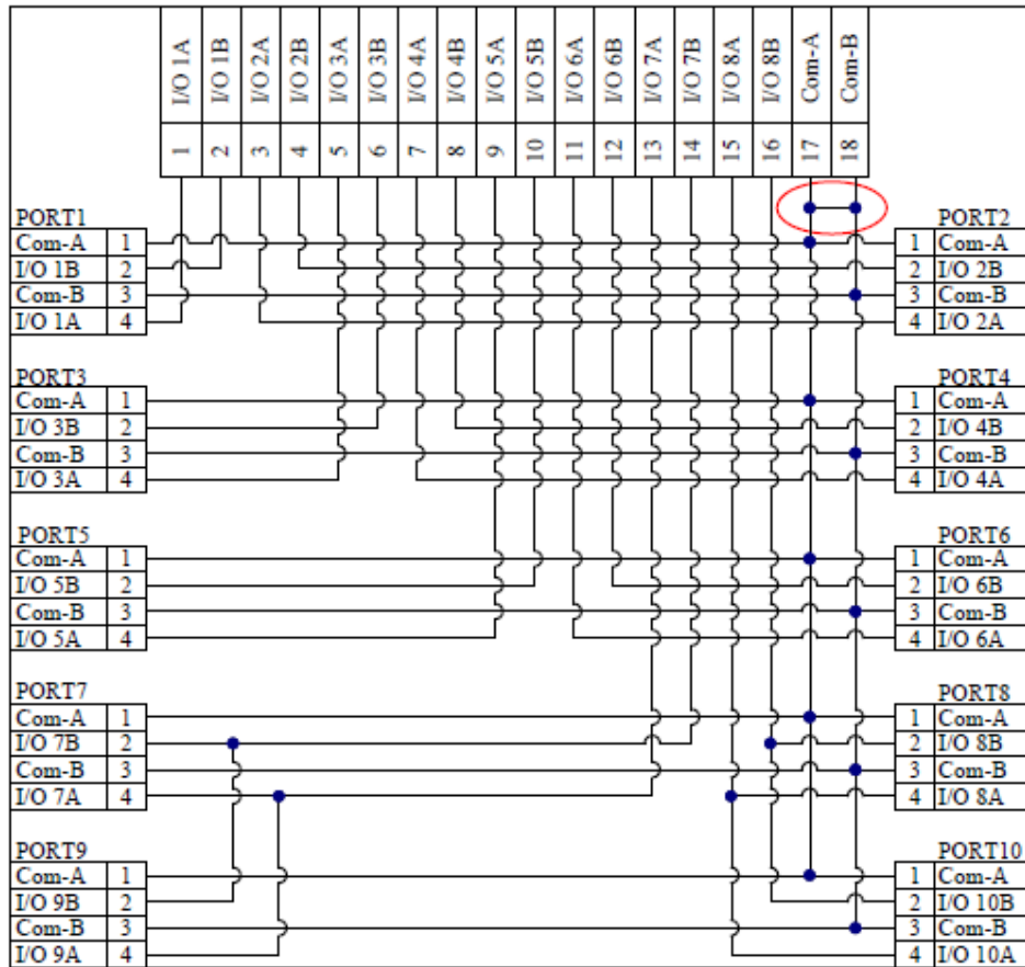
34045-3-000 I/O Diagram
