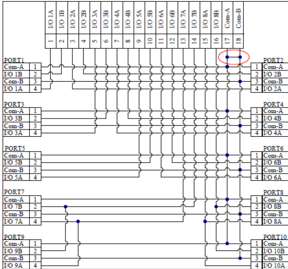
34045-5-000 I/O Diagram
